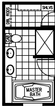
'CUBBY' BATH OPT W/72" SOAKER TUB AND 48" SHOWER
