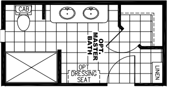
DELUXE BATH W/CORNER TUB, 60" SHOWER AND DRESSING SEAT
